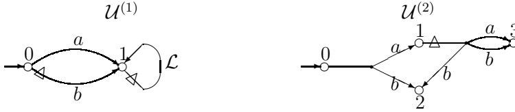
Fig. 2. Two Underspecified Transition Systems
