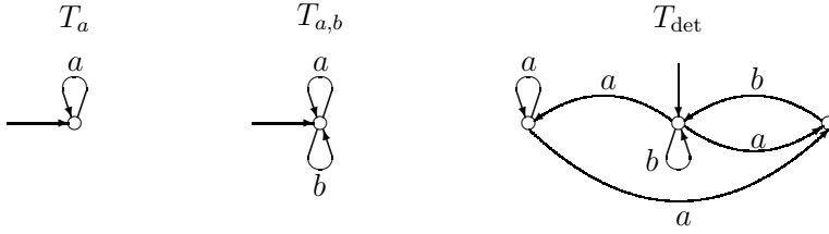
Fig. 1. Some Transition Systems
