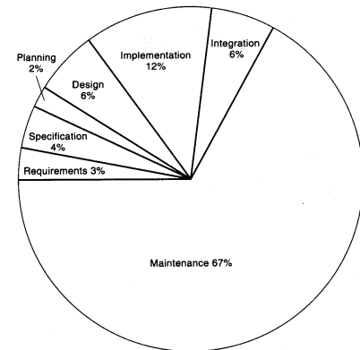
Figure 1.2 Approximate relative costs of phases of software production process.
