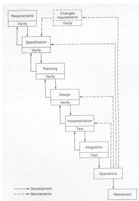
Figure 2: Life-cycle phases of waterfall model
