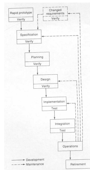
Figure 3: Life-cycle phases of rapid prototyping model
