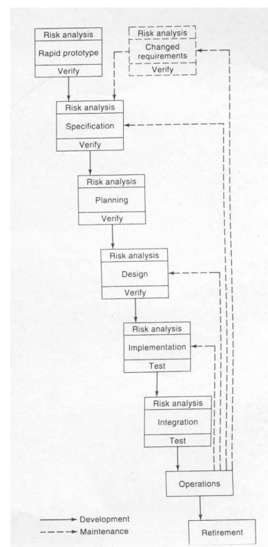
Figure 4: Life-cycle phases of spiral model
