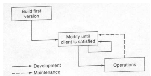
Figure 1: Life-cycle phases of build-and-fix model
